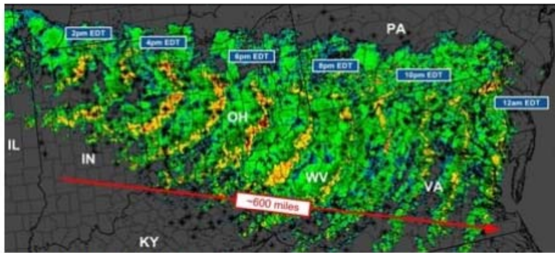
Radar sequence of derecho thunderstorm complex. Storm traveled about 600 miles in 10 hours at an average speed of 60 mph. (Storm Prediction Center)
