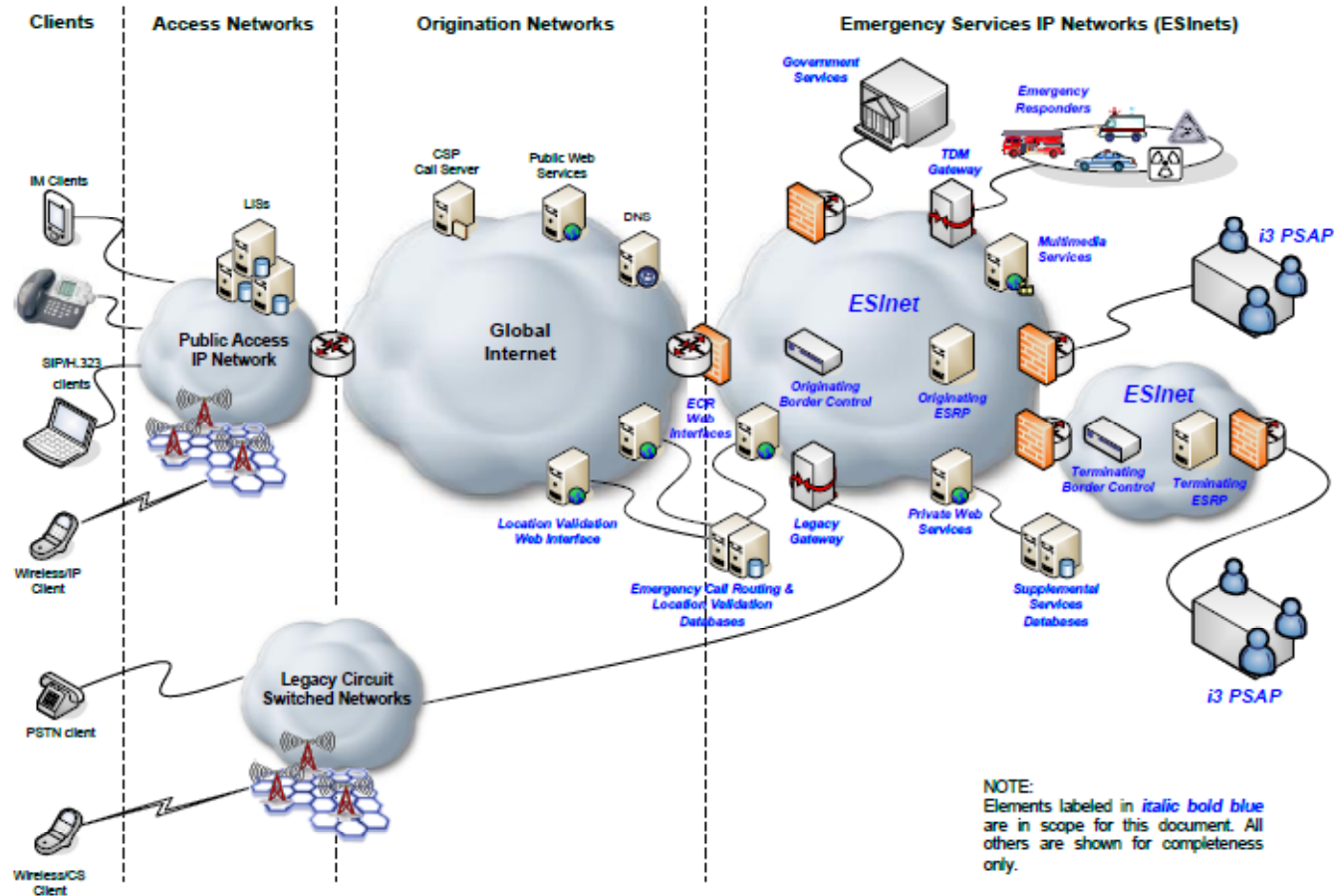
Figure 4-3 Example i3 Physical Architecture
